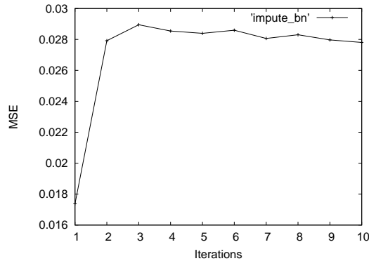
Fig. 2. Results of algorithm IMPUTE_BN for database housing with 10 iterations
