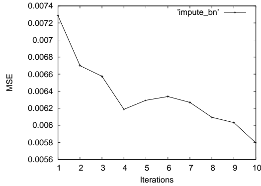
Fig. 3. Results of algorithm IMPUTE_BN for database water with 10 iterations
