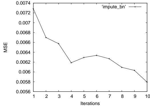
Fig. 1. Results of algorithm IMPUTE_BN for database chest with 10 iterations
