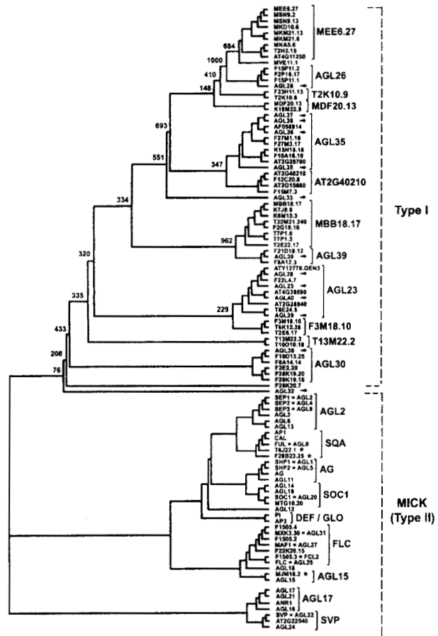
Fig. 2. Phylogenetic analysis of the MADS-box family in Arabidopsis . A total of 104 protein sequences comprising the MADS-box plus some 20 - 50 additional residues were aligned using the Clustal X (v.1.8) program using the default settings. The alignment containing 120 positions was used to construct the unrooted neighbor-joining tree. Clusters for Type II factors were designated as in (Theissen et al. 1996), or arbitrarily, for the Type I class. Arrows indicate those Type I factors already cited in literature. Type II factors not previously reported are marked by an asterisk. Bootstrap values (over 1000 replicates) are indicated for relevant nodes of the Type I class. MADS-box proteins not previously reported were named according to their gene designation as stated in the Arabidopsis databank.
